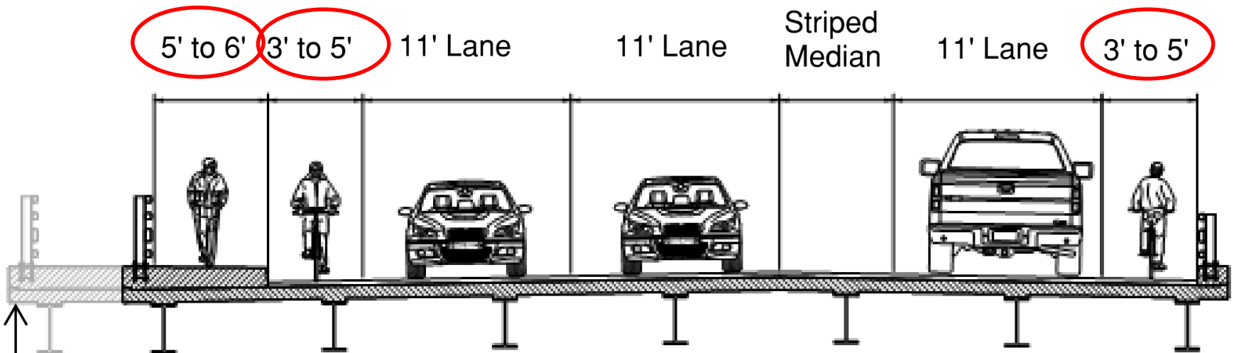
BRIDGE OPTION W/ SIDEWALK
