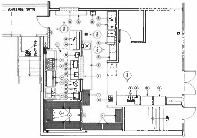
1. Equipment Schedule Plan 1/4" = 1'-0"
