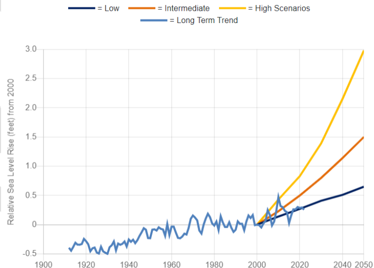
Annual Sea Levels Referenced to 2000, NOAA Station 8418150, Portland 1912-2022
