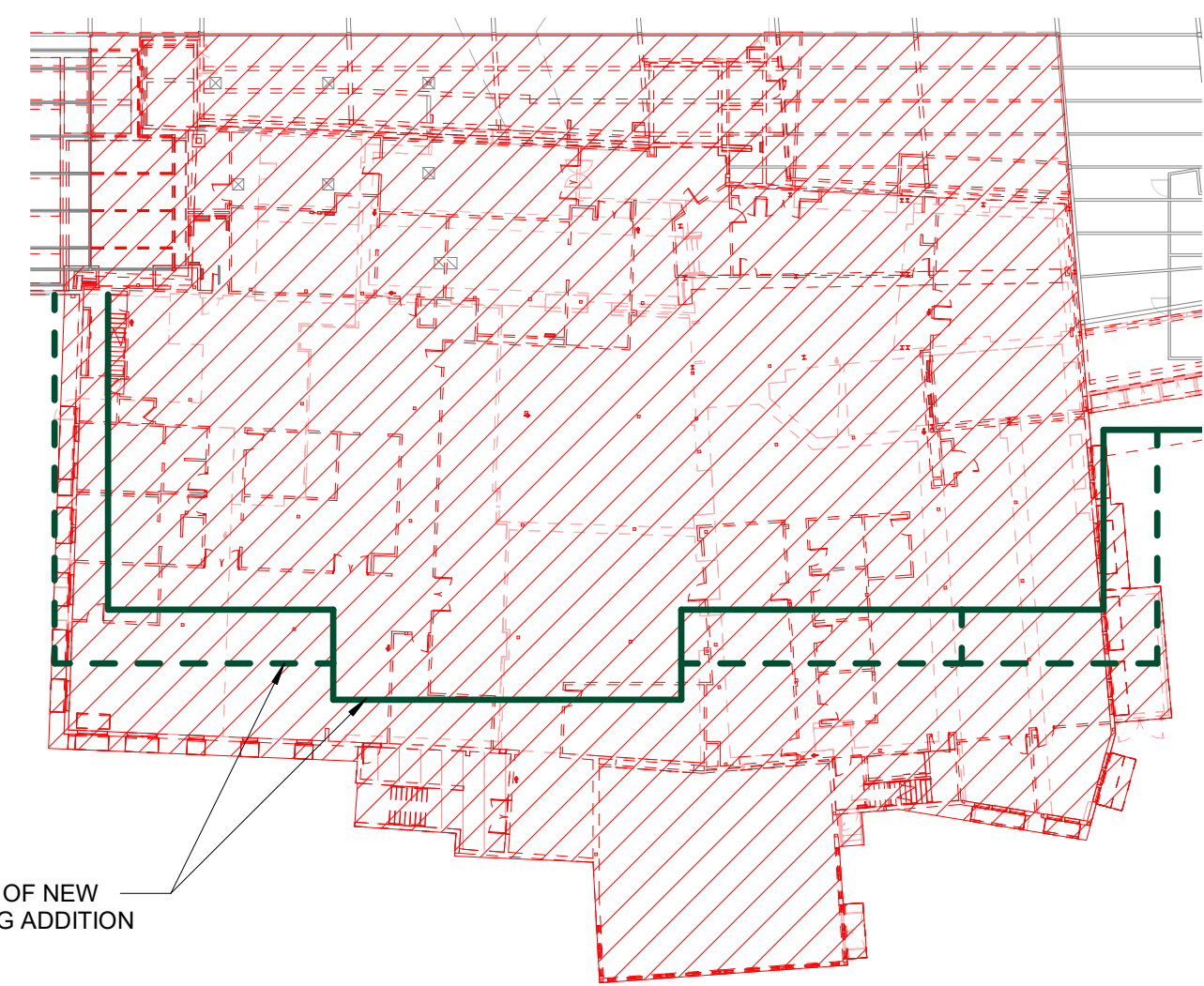
3 SANDWICH FLOOR REMOVALS PLAN 1/32" = 1'-0"
