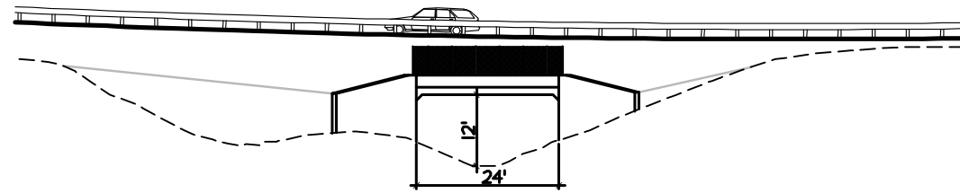
ELEVATION SCALE 1"=10'
